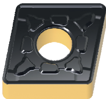
RA基本形状C型 C type inserts with RA chip breaker
