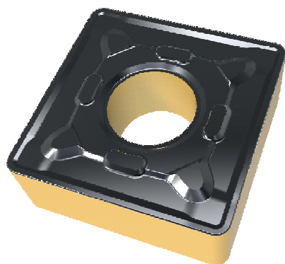
RA基本形状S型 S type inserts with RA chip breaker
