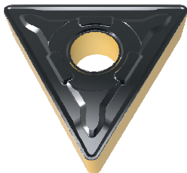
RA基本形状T型 T type inserts with RA chip breaker
